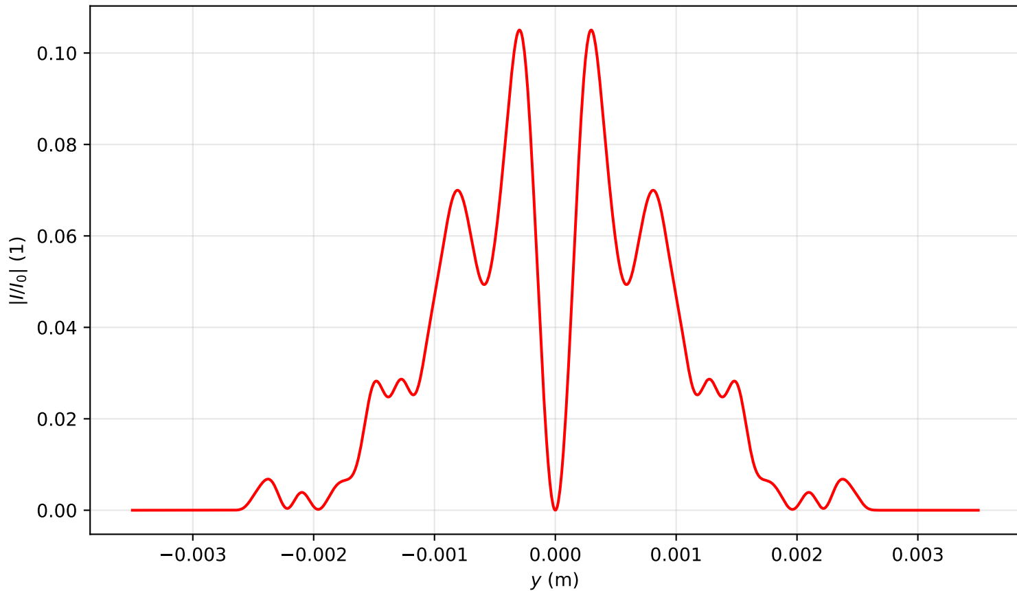
Intensity profile I(x=0, y, z=2.309)/I_0 , P_{in}=8.0P_{cr} , artificial time
